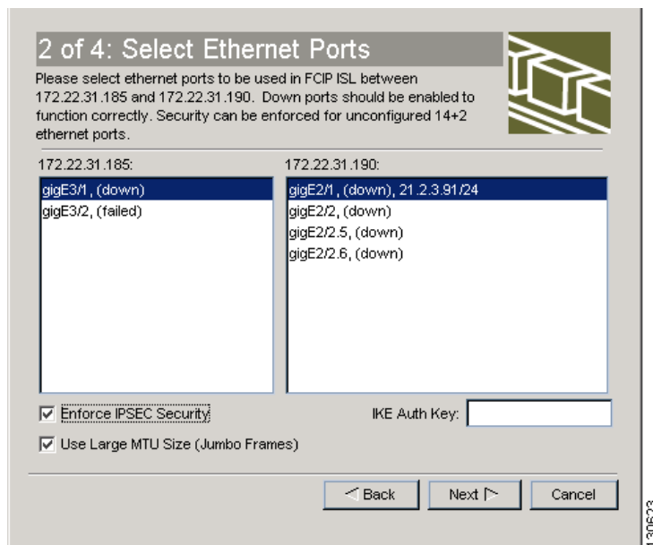
Figure 19-5 Enabling IPsec on an FCIP link
